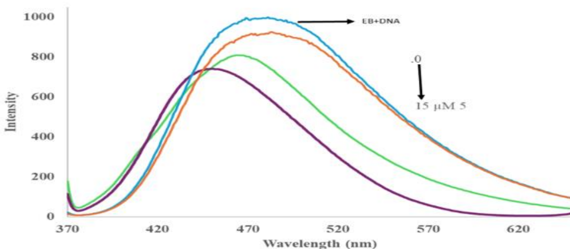
Fig. 8: Emission spectra of addition of increasing amount of 5 complex (0, 5, 10 and 15 \mu\text{M} ) to EB+DNA complex (blue line).
